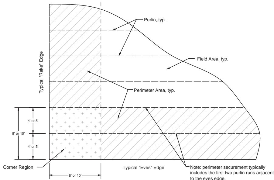
Metal Roofing Retrofit - Detail at Perimeter/Corner
